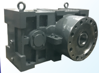
EXTRUDER HELICAL GEAR BOX
